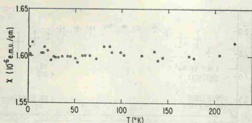
FIG. 4. The magnetic susceptibility of \alpha -U from 1–200°K. The value observed at 297°K was 1.645 \pm 0.030 \times 10^{-6} emu/gm.
